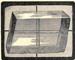
Iceland Spar or Double refracting Spar.
